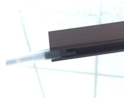
5. Let the new LED strip slide into the rib.
