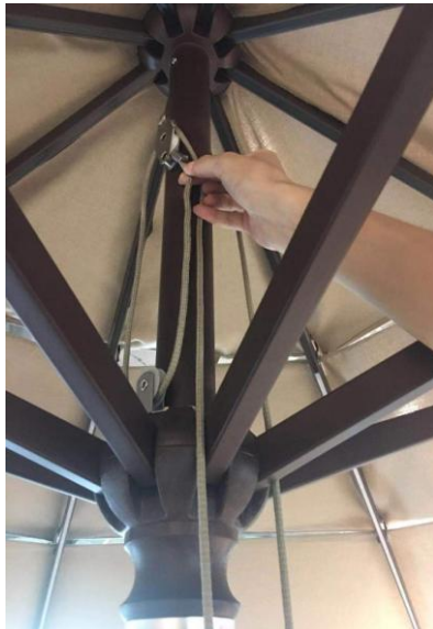
4. Go through the underside of upper pulley and tie a knot. Please note the knot is Flemish knot.
