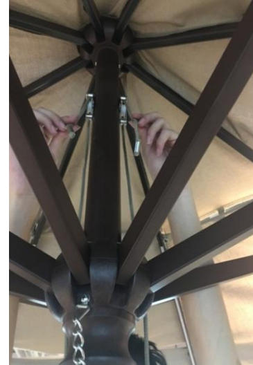
2. Let the cord go through the upside of upper pulley and pull the cord down. (The cord has two ends, and one end goes through one pulley.)
