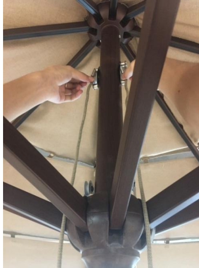
2. Let the cord go through the upside of upper pulley and pull the cord down. (The cord has two ends, and one end goes through one pulley.)
